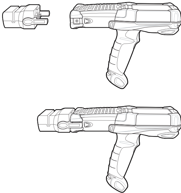
Figure 5-7 Attaching the MSR
