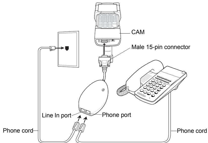
Figure 5-18 Modem Dongle Connection - MC92N0-G
