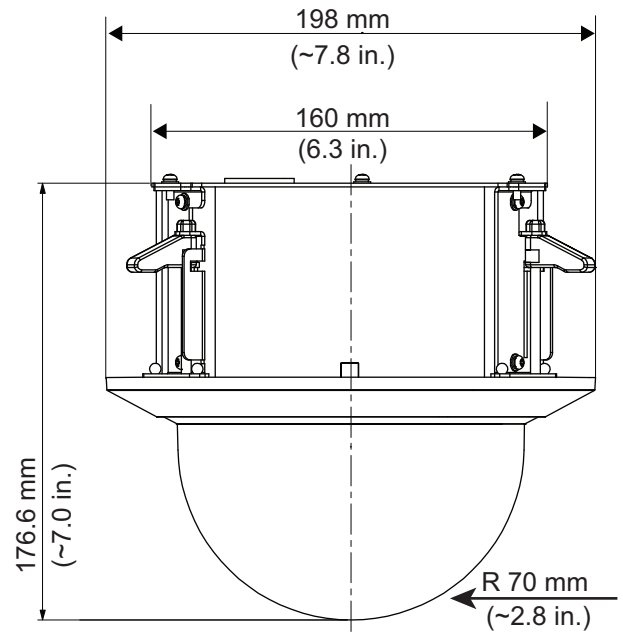
Fig. 6: In-ceiling model
