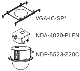
Fig. 5: In-ceiling mount
