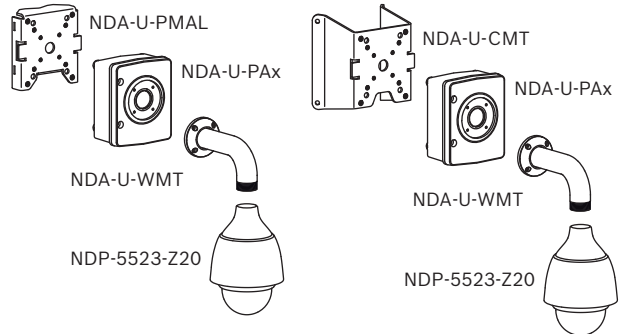
Fig. 3: Pole mount (IP66); Corner mount (IP66)
